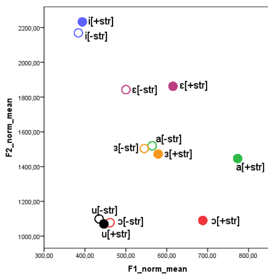
Figure 1: Group average F1/F2 vowel plot
